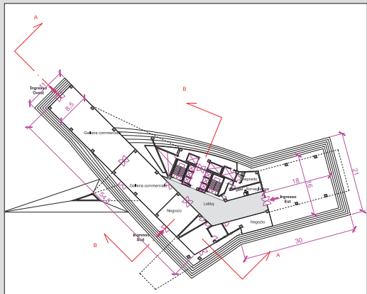
Piano Terra 1:500
