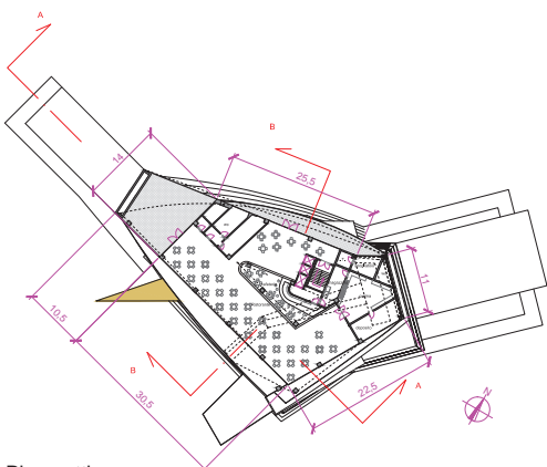
Piano attico
